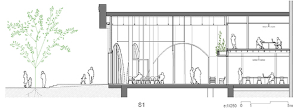
S1 e:1/250 0 1 5m
