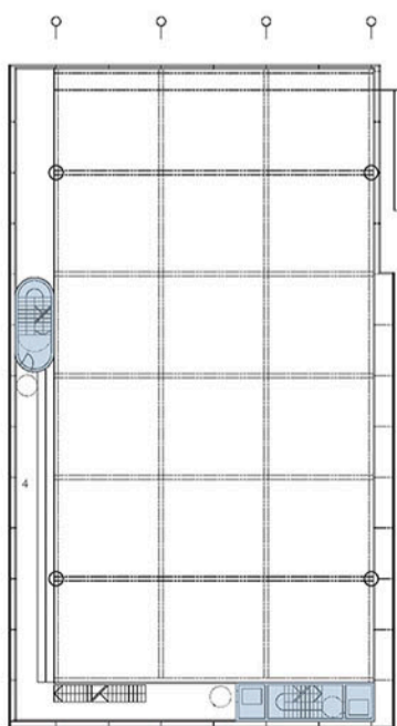
P1 Planta Grades pista 1 + 8.65 m E/1:300
